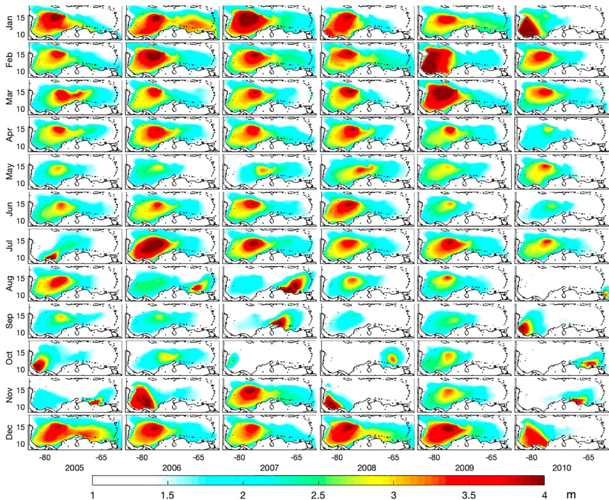
FIGURE 7 Monthly H_s^M distribution (in m) in the Caribbean Sea for the period of 2005 to 2010.
