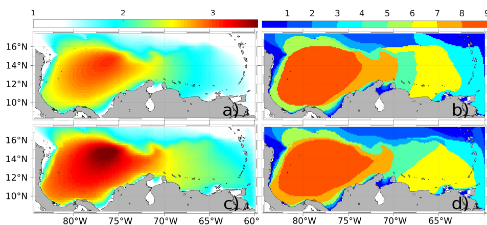
FIGURE 3 Mean value of extreme wave heights in the basin (units in m) (A, C) and regionalization from the 3 \times 3 SOM temporal analysis (B, D) where each region (R1–R9) corresponds to the output of a neuron. Top figures correspond to H_s^M and bottom figures to H_s^{99} .
