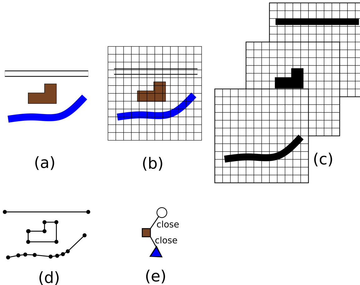
Figure 1: Different types of location encoding for cartographic data. a) Cartographic data to encode (vector + symbols); b) raster encoding; c) layered raster encoding; d) graph encoding; e) spatial relations encoding.
