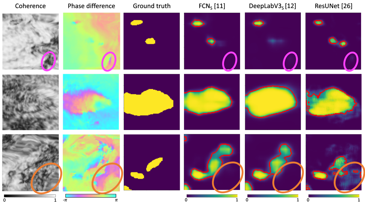
Fig. 3: Qualitative comparison of the predictions of FCN_S [11], DeepLabV3 _S [12] and ResUNet [26] which shown the best quantitative results. Red borders denote the segmentation used to calculate Table I results. Magenta circles illustrate a suspicious pattern in the phase difference map but with a low coherence identifying an unreliable pattern. Orange circles identify an area with strong layover distortions.
