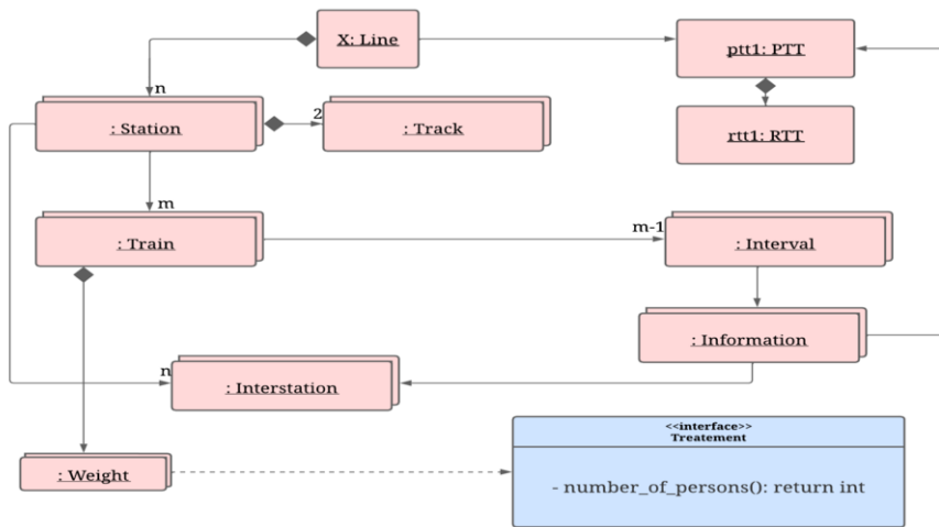
Figure 7. Object diagram representing the raw data.
