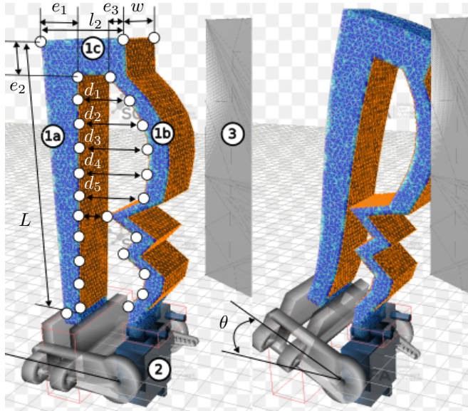
Fig. 1. Illustration of the finger design parameterization. Finger composed of left (1a), top (1c), and right (1b) walls. (2) Servomotor. (3) Example of object to grasp, fixed in space. Left: rest configuration. Right: closed configuration.
