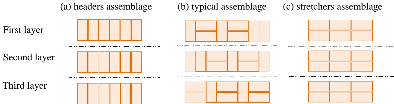
Figure 5: Top view of three different assemblages with headers and stretchers. (a) An assemblage using only headers. (b) A typical assemblage respecting the standards of dry stone construction. (c) An assemblage using only stretchers.
