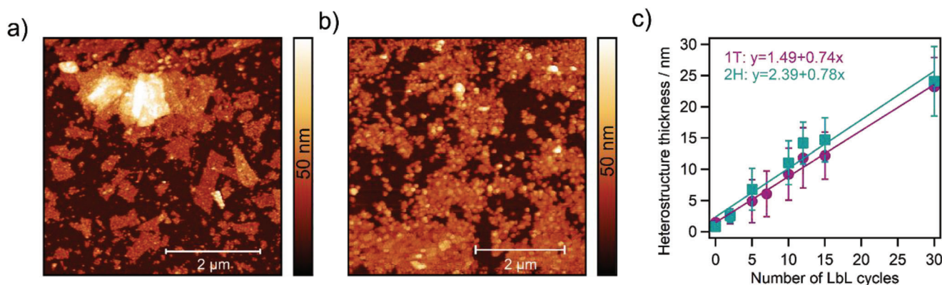
Figure 2. AFM topography of the heterostructure a) HTCP(x15)/1T and b) HTCP(x12)/2H. c) Linear dependence between the number of LbL immersion cycles and HTCP/MoS 2 thickness.
