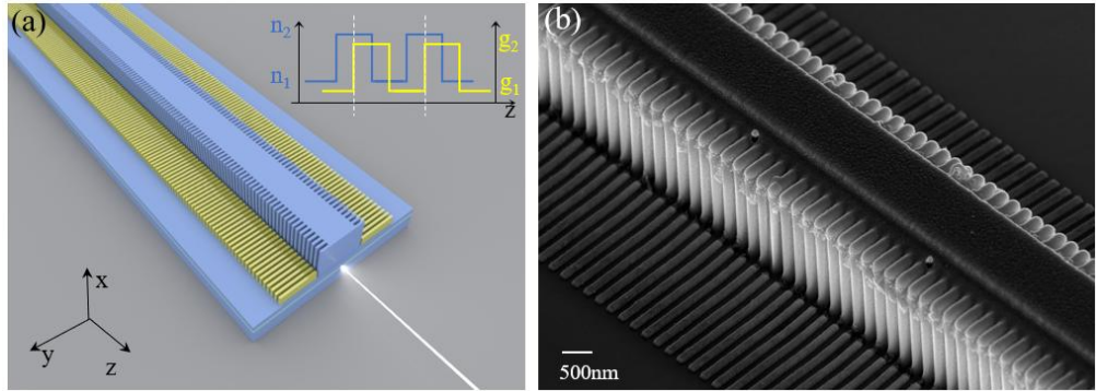
Fig.1. (a) Sketch of PT-symmetry DFB laser, blue (dielectric) and yellow (metallic) gratings are shown; the inset depicts the condition for PT symmetric potential. (b) SEM side view of a fabricated first-order PT-symmetry DFB laser.
