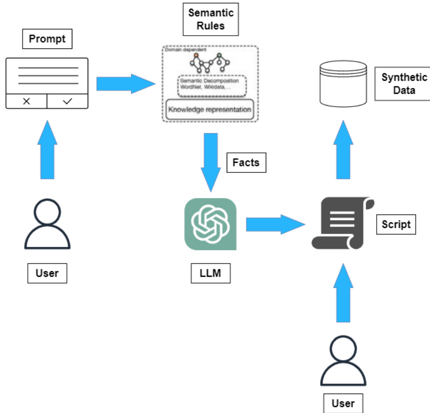
Fig. 1 High-level architecture of neuro-symbolic synthetic data generation workflow
