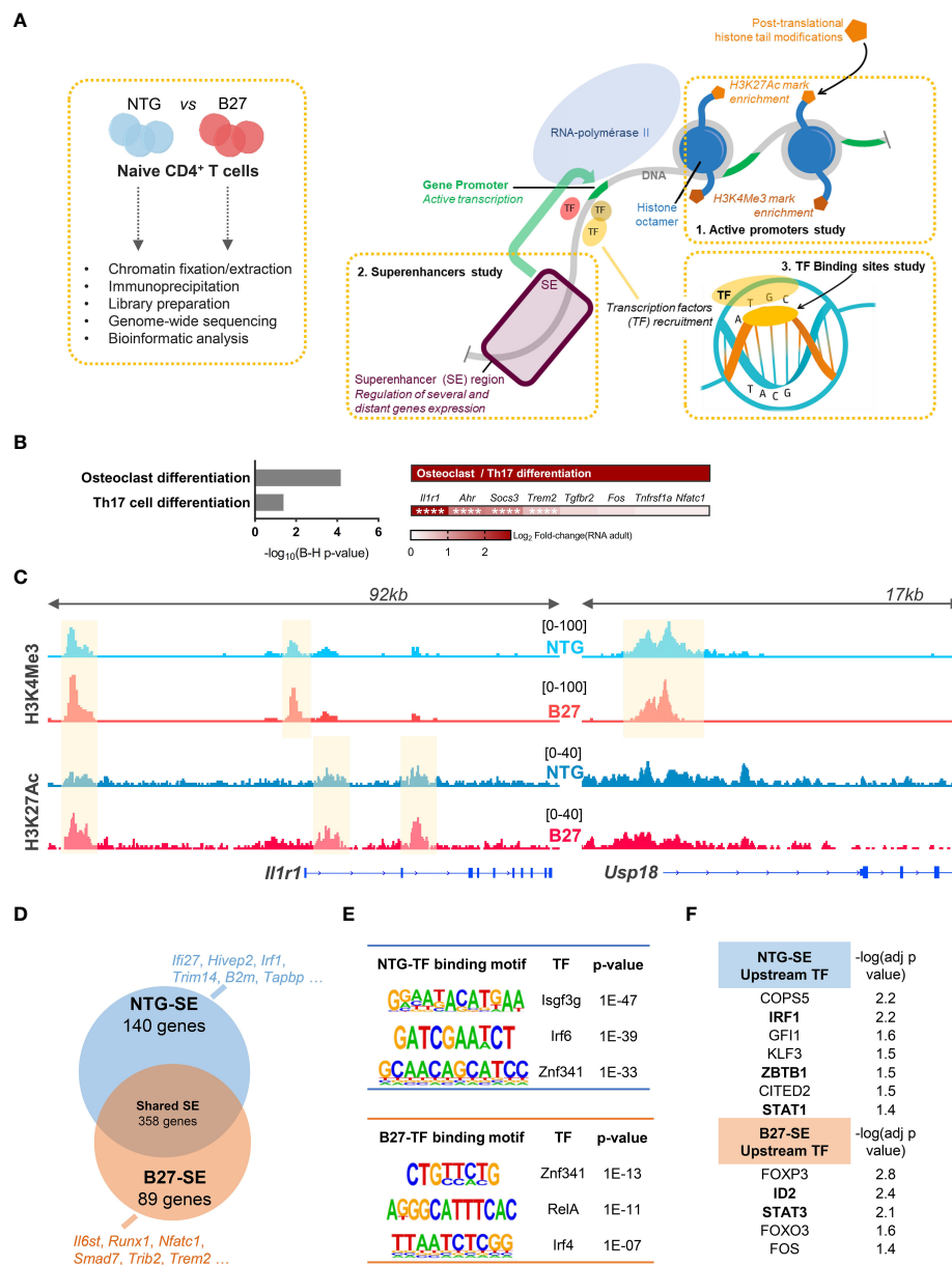
FIGURE 3 Th17 imprint of B27-rat Tn is epigenetically determined. H3K4Me3 and H3K27Ac activating HM ChIP-seq on mLN Tn from 3-month-old sick B27-rats and age-matched NTG littermates ( n = 3 ). (A) Cartoon recapitulating the steps of ChIP-seq experiments and the features profiled: active promoters, superenhancers regions and binding transcription factors. (B/Left) KEGG pathways enriched for genes harboring a differential peaks enrichment of H3K4Me3 and/or H3K27Ac histone marks, in B27-rats compared to controls. (B/Right) Both KEGG pathways included the notified genes, and \text{Log}_2\text{FC}(\text{RNA}) refers to the relative gene expression in Tn from B27-rats, as compared to controls from RNA-seq dataset. **** adjusted p < 0.0001 . (C) Integrated genome viewer snapshots of genes involved in Th17 ( Il1r1 ) and IFN ( Usp18 ) pathways. Differentially enriched peaks at gene promoter (H3K4Me3) and/or presumed gene-related enhancer (H3K27Ac) are highlighted in yellow. Dataset from one pair of B27/NTG rats, representative of three. (D) Venn diagram showing the genes at proximity of the SE specific of B27-rat Tn and those specific of NTG littermates (using ROSE algorithm). Examples of SE-related genes specific of NTG and B27-rat Tn, involved in IFN (blue) or Th17 (red) pathways. (E) Examples of de-novo binding motifs of transcription factors predicted to fix on either NTG or B27-SE (using HOMER). (F) Upstream transcription factors predicted to regulate the expression of NTG or B27-rats SE-related genes (using IPA). -\log(\text{adj } p\text{-value}) calculated by Fisher's exact test. Transcription factors in bold if the transcript relative expression (foregoing RNA-seq data) was either decreased (NTG SE) or increased (B27-SE) in pre-morbid and sick B27-rat T cells relative to controls.
