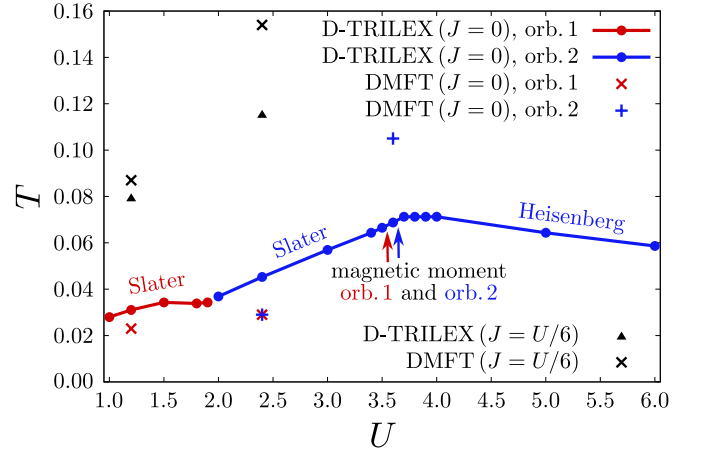
FIG. 1. Néel temperature for the two-orbital half-filled Hubbard model on a cubic lattice with different bandwidths of the two orbitals. Results are obtained using D-TRILEX and DMFT for different values of the Hund’s exchange coupling J . At finite J the Néel transition occurs simultaneously for both orbitals (black “▲” and “×” markers). The OSNT scenario is realized in the absence of J : at U < 1.95 upon decreasing the temperature the Néel transition occurs first for the narrow orbital (orb. 1, red color), and at U > 1.95 for the wide orbital (orb. 2, blue color). Critical interactions at which the local magnetic moment is formed above the Néel transition are indicated by arrows.
