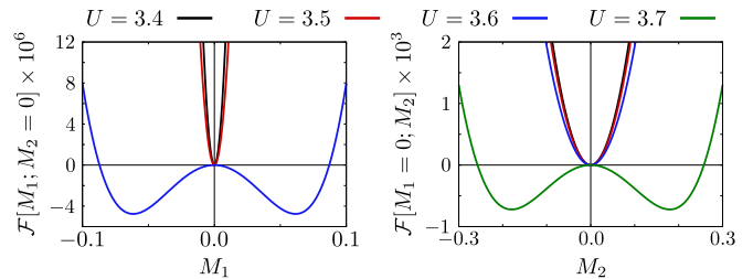
FIG. 3. Local free energy \mathcal{F}[M_1; M_2] as a function of the value of one of the two local magnetic moments M_1 (orb. 1, left panel) and M_2 (orb. 2, right panel) obtained along the Néel phase boundary. The transition from a parabolic form of the free energy to a double-well potential form signals the formation of the local magnetic moment, which for both orbitals occurs approximately at the same value of the interaction U = 3.55 (orb. 1) U_2 = 3.65 (orb. 2).
