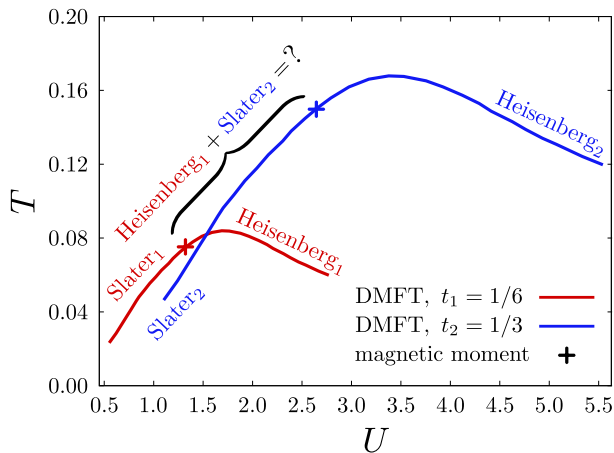
FIG. 2. Sketch of the proposed mechanism for the OSNT. Red and blue curves show the Néel phase boundaries predicted by DMFT for a half-filled single-band Hubbard model on a cubic lattice as a function of the local interaction strength U . Results are taken from Ref. 109 and rescaled to get the phase boundaries for two different bandwidths defined by the nearest-neighbor hopping amplitudes t_1 = 1/6 (red) and t_2 = 1/3 (blue). “+” markers indicate the point on each phase boundary at which the local magnetic moment is formed (see Ref. 96), which separates the Slater (at smaller U ) and Heisenberg (at larger U ) regimes of the Néel transition.
