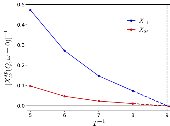
FIG. 4. Temperature dependence of the inverse of the X_{11}^{sp} and X_{22}^{sp} orbital components of the static ( \omega = 0 ) spin susceptibility X_{ll}^{sp} calculated at the antiferromagnetic wave vector Q = \{\pi, \pi\} . Results are obtained for the two-orbital Hubbard model on a square lattice considered in Ref. 56 with t_1 = t_2 = 1 , t'_1 = 1 , t'_2 = 0 , U = 4 , and J = 1 . The vertical dashed line at T^{-1} = 9 indicates the Néel transition point at which both components of the spin susceptibility diverge. The transition point was obtained by a linear extrapolation of the results (dashed blue and red lines).
