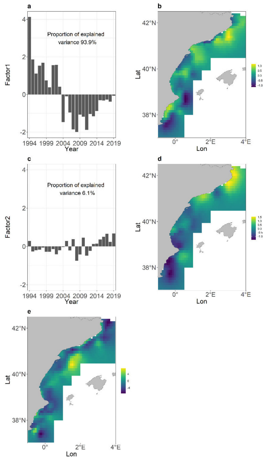
Fig. 2. Portrayal of (a, c) the two dominant modes (factors) of density spatiotemporal variability for the Spanish Coast (GSA06), (b, d) the spatial maps associated with the two modes, and (e) the spatial variation \omega , which depicts the long-term average spatial pattern of red mullet density. For each axis (a, c), the proportion of explained variance is indicated. In panels b and d, yellow and blue tones represent areas that are associated with the positive and negative phases of the mode of variability, respectively. In panel e, yellow and blue tones represent high- and low-density areas. Map projection is WGS84 UTM.
