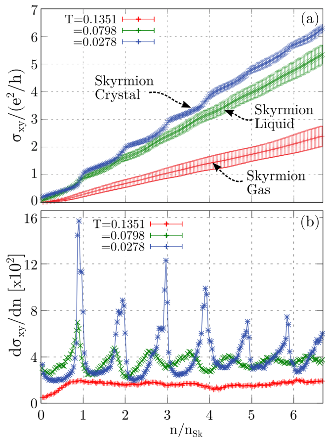
FIG. 15. (a) Hall conductivity \sigma_{xy} as a function of doping n for T/t = 0.1351, 0.0798, and 0.0278 , which correspond to SkG, SkL, and SkX regions, respectively. The electron density n is scaled with the skyrmion density n_{\text{Sk}} \equiv 2.2425 \times 10^{-3} of the SkX phase. Namely, n/n_{\text{Sk}} = 1 means an electron density just filling up the lowest skyrmion band. (b) Derivative of \sigma_{xy} with respect to doping n . The Hall conductivity quantization appears as peaks in the SkX and SkL regimes, but disappears in the SkG region (except for a weak signal at very low doping). The change of periodicity of the peaks between the SkX and SkL is due to the decrease of skyrmions with temperature.
