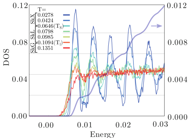
FIG. 16. A set of one particle electron density of states (DOS) is shown for several temperatures across T_s and T_l . To facilitate the comparison of oscillation amplitudes, we shift energies to each curve to place the lowest peak at the same position. After this shift, we set the origin of the energy near the band bottom. We also show the accumulated density of states at T = 0.0278 . The thin horizontal lines are integer multiples of n_{\text{Sk}} to compare with the accumulated DOS.
