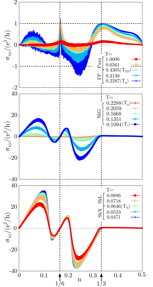
FIG. 14. Hall conductivity \sigma_{xy} as a function of doping n (top) around T_{\text{FP}} , (middle) between T_g and T_l , and (bottom) around T_s . Please note that the different scale of longitudinal axis in the top panel. For the guide to eye, we draw vertical dashed lines to indicate n = 1/6 and n = 1/3 , and horizontal dashed lines to indicate the quantized Hall conductivity.
