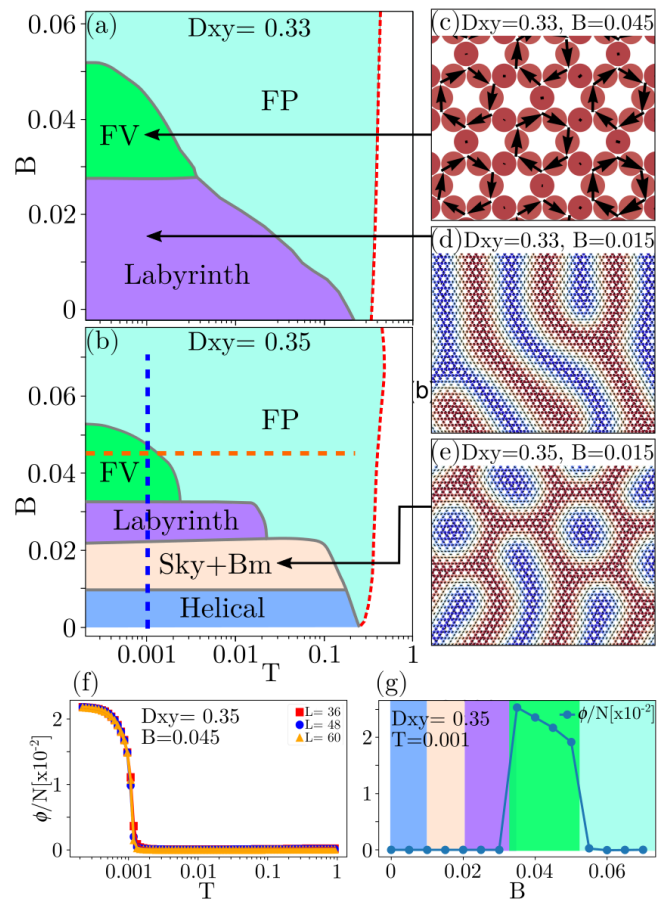
FIG. 4. B vs T phase diagrams for D^z = \sqrt{3} and D^{xy} = 0.33 (panel (a)) and D^{xy} = 0.35 (panel (b)) with representative spin configurations (c-e) (lattice size L = 48 ). In panel (f) we present the order parameter \phi (scaled by system size N ) as a function of temperature for three different system sizes L = 36, 48, 60 for D^{xy} = 0.35 and magnetic fields B = 0.045 . Panel (g) presents the evolution of \phi as a function of the magnetic field B showing a well-defined region where the FV phase emerges. In panels (f) and (g) the error bars are the size of the markers.
