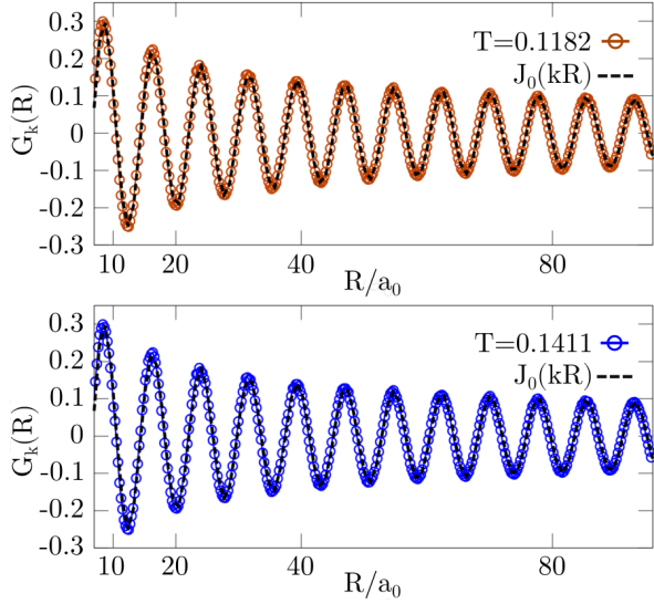
FIG. 11. Positional correlation function calculated for \langle G_{|K|}(R) \rangle (dashed black line) and G_K(R) from MC simulations at fixed magnetic field B/J = 0.09 . For both temperatures the system is in the SkG phase.
