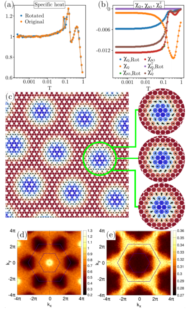
FIG. 12. Top: Comparison of specific heat (a), nearest neighbor chirality \chi_Q , third nearest neighbor chirality \chi_Q^{N3} and plaquette chirality \chi_Q^T (b) as a function of temperature for the original (Eq. (1)) and rotated (Eq. (9)) Hamiltonians. (c) Low-temperature spin configuration of the SkX lattice (left) and for each sublattice (right). Comparison of the magnetic structure factor S^\perp in the spin-liquid regime at T = 0.1853 between the (d) original and (e) rotated Hamiltonians. All data have been measured for D^{xy} = 0.5 and B = 0.09 (lattice size L = 48 ).
