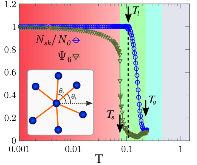
FIG. 9. Competition between the chiral spin liquid and skyrmion solid at B = 0.09 as measured from: (a) the specific heat C_h and magnetisation M_z , (b) the normalised number of skyrmion N_S and orientational order parameter \Psi_6 of Eq. (4) whose angle \theta_{ij} is defined in the inset. N_0 is the saturated number of skyrmions for B = 0.09 . (Figure taken from Ref.[31])
