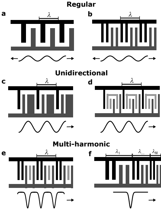
FIG. 14: Interdigital transducer designs.
