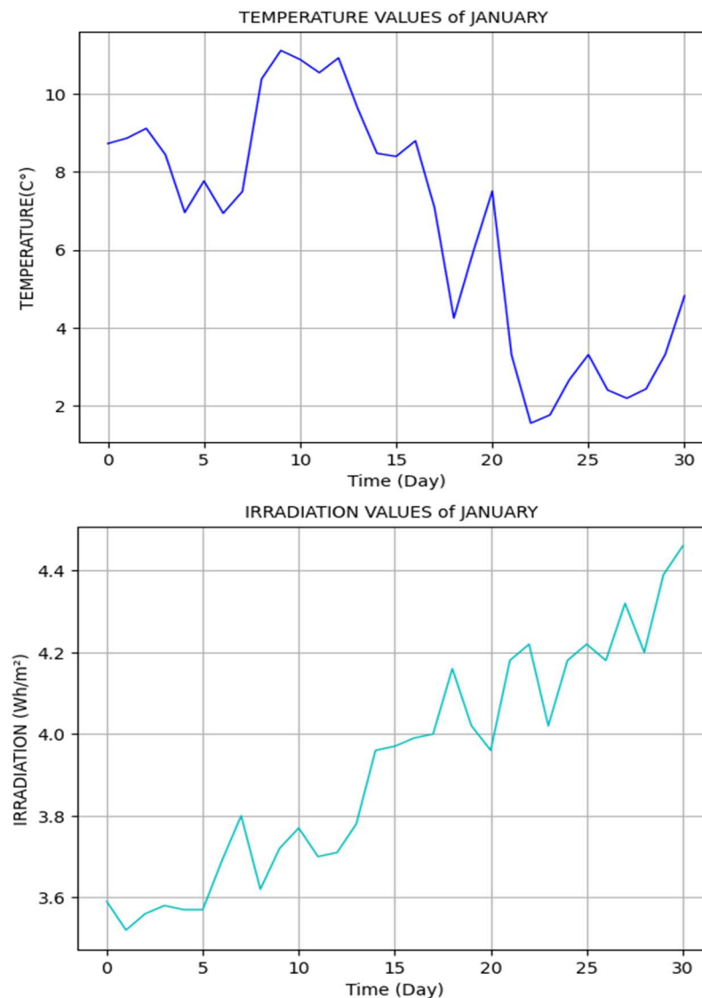
Figure 8. The dataset from the month of January in Hassi R'Mel used in this study is presented as follows: (Top) the daily average temperature recorded per day, (Bottom) the daily solar irradiance data for the month of January.
