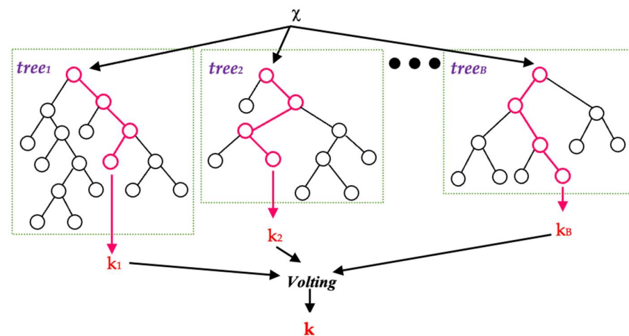
Figure 2. An example of the random forest model’s algorithm.
