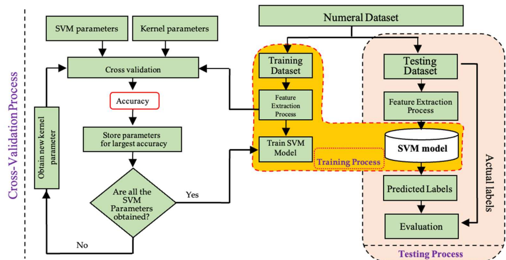
Figure 3. Schematic description of the SVM model algorithm.
