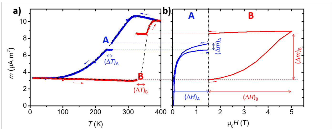
Fig. 4 (a) m(T) curves measured at a magnetic field of 1.5 T. The dashed m(T) curve is measured under continuous temperature sweeping. The blue m(T) curve is measured upon cooling, and interrupted with a m(H) loop at 250 K (step A). The red m(T) curve is measured upon heating, and interrupted with a m(H) loop at 325 K (step B). (b) Irreversible m variation, when decreasing the field H over (\Delta H)_A (step A), and when increasing the field H over (\Delta H)_B (step B).
