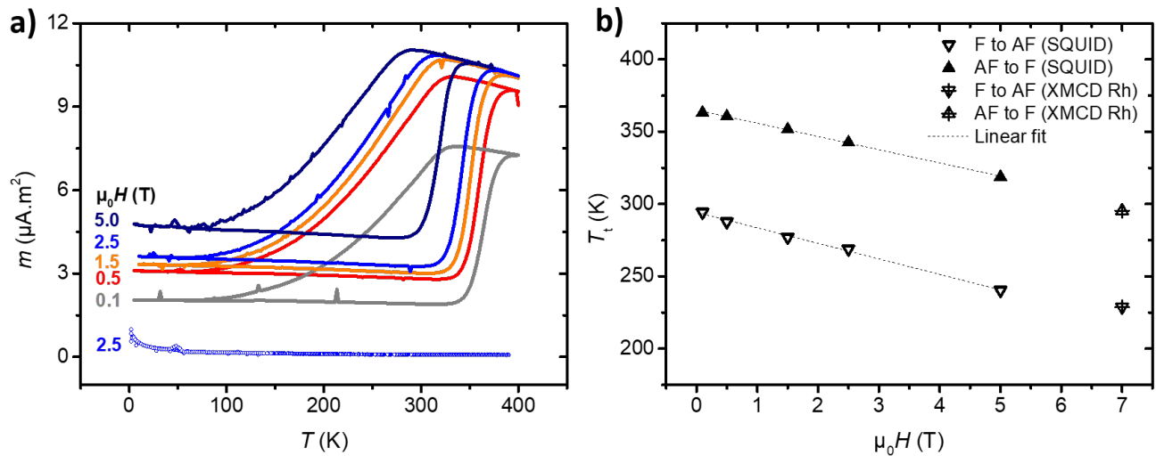
Fig. 3 (a) SQUID magnetometry between 4 K and 400 K for external magnetic field of 0.1 T (grey), 0.5 T (red), 1.5 T (orange), 2.5 T (blue) and 5.0 T (dark blue). The m(T) curves measured after annealing are represented with full symbols, and compared to the m(T) curve measured at 2.5 T in the as prepared state (open symbols). (b) The transition temperature determined from SQUID m(T) curves, in the cooling-down branch (upside-down open triangles) and the heating-up branch (filled triangles) calculated as the maximum of the first derivative. The dashed lines are best linear fits. The points at 7 T are obtained from the XMCD signal on Rh edge.
