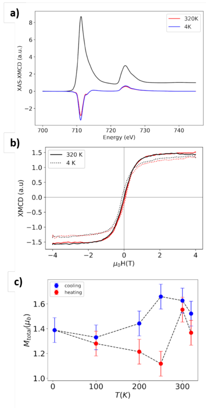
Fig. 6 XAS and XMCD in the soft X-ray regime measured on the annealed FeRh nanocluster assembled film at the Fe L-edge in TEY mode under 6 T and perpendicular incidence leading to a total magnetic moment of 1.4 \mu_B at 4 K and 1.5 \mu_B at 320 K (a). XMCD signal taken as the max XAS value at the Fe L_3 edge versus the applied magnetic field (b). Temperature dependence of the Fe total magnetic moment measured from the thermal XMCD evolution under 6 T (c).
