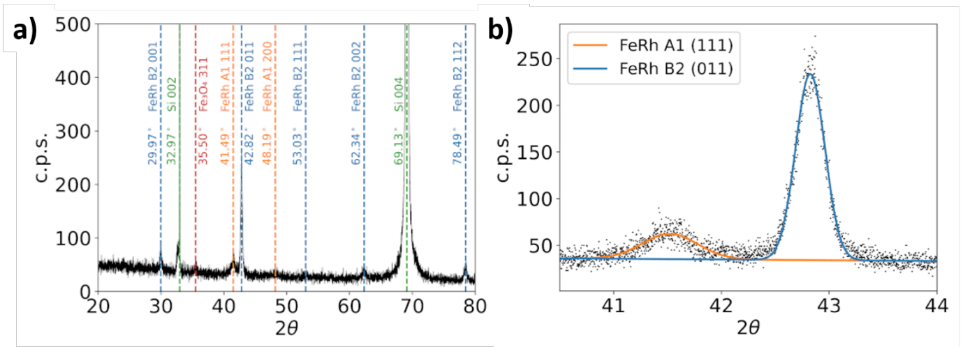
Fig. 2 Specular XRD pattern of the FeRh nanocluster assembled film with labelled peak positions of FeRh A1 phase (orange), FeRh B2 phase (blue), Si (green) and \text{Fe}_3\text{O}_4 (red) (a). Magnification of the XRD pattern in the region of FeRh A1 (111) and FeRh B2 (011) peaks with Gaussian fits using the Scherrer formula with shape factor 0.9.
