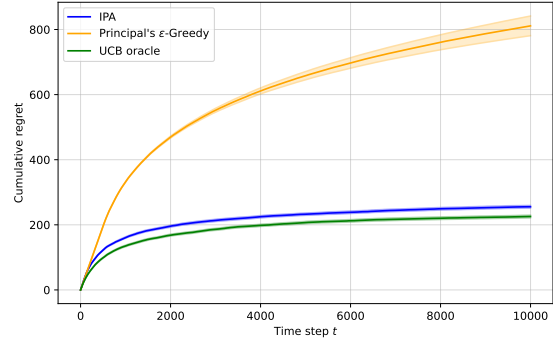
Figure 2: Cumulative regret for different algorithms on a 5 arms instance.
