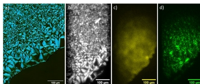
Figure 12. Polarized optical image of compound ( S )-BPM-3,5-C4(1) obtained through optical microscope (a). Polarized bright field image obtained with a polarized LED source recorded on the iCCD camera (b). MPF (c) and SHG (d) images illuminated with an incoming s -polarized laser source at a laser power of 510 mW.
