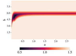
Fig. 4. Heatmap of the distance to \gamma .
