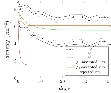
Fig. 2. \varphi_- -accepted, \varphi_+ -accepted and rejected simulations.
