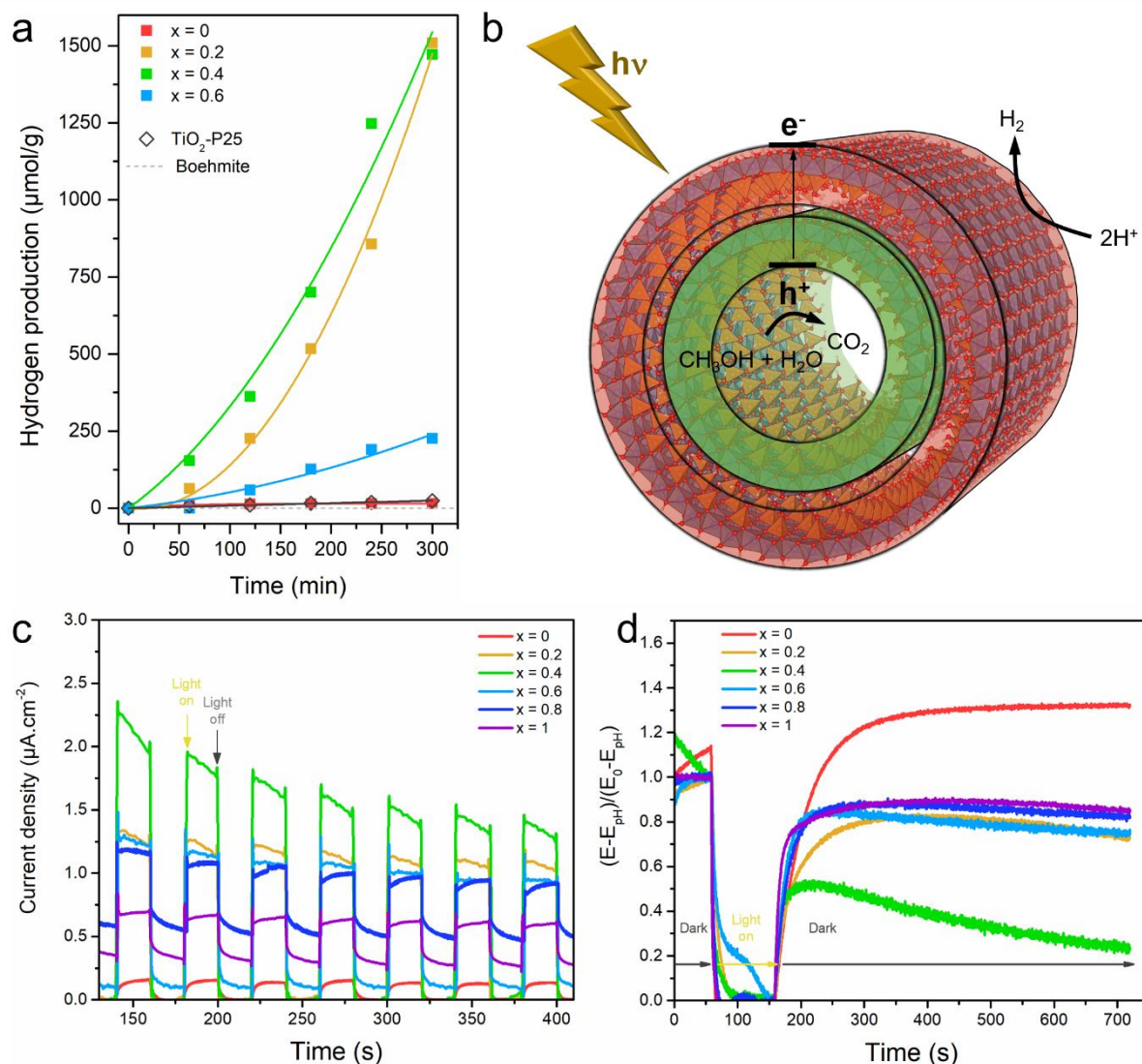
Figure 6. Hydrogen evolution reaction under solar-light irradiation for (a) Ge-DWINT and Ti/Ge samples with different ratio. The \text{H}_2 production by standard \text{TiO}_2 (P25) and boehmite nanoparticles are also reported for comparison. (b) Schematic illustration of the proposed \text{H}_2 production mechanism, pointing out the general steps involving electron/hole charge separation/reaction pathways. (c) Transient photocurrent response and (d) normalized open-circuit voltage-decay curves of Ti/Ge samples.
