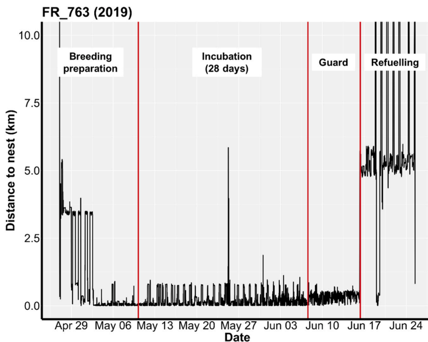
Fig. 2. Distance between each recorded GPS fix and the nest during the breeding season, used to distinguish the different key stages of a typical curlew breeding cycle.
