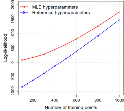
(b) Log-likelihood
