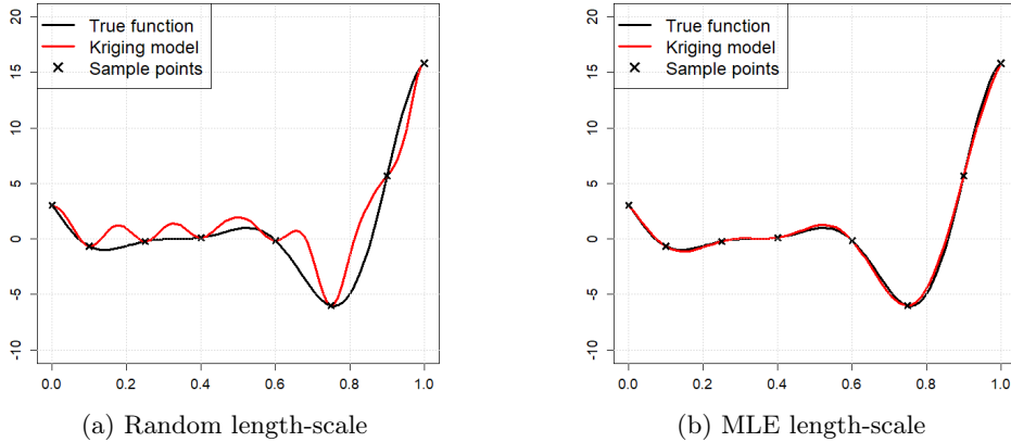
Figure 1: Example of an ordinary Kriging model in 1D. Left: model with an arbitrary length-scale \theta = 0.03 , right: model with length-scale obtained by MLE.
