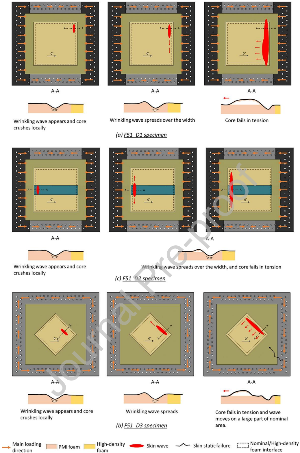
Figure 30. Failure scenario for specimens under compression and shear.
