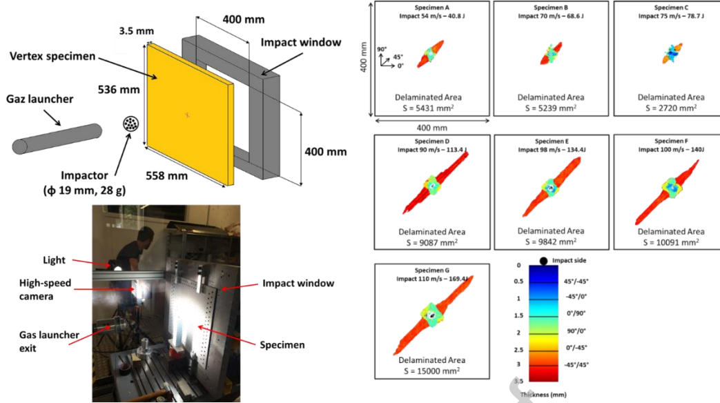
Figure 24. Impact test set-up and Delamination areas obtained by C-Scan after impact for the seven specimens
