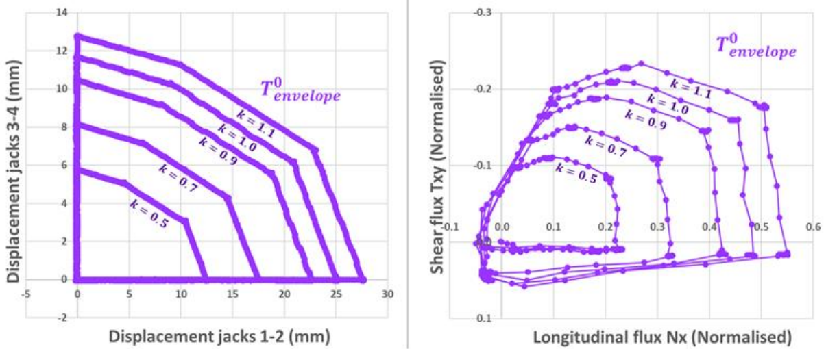
Figure 34: Representation of the T^0_{envelope} test through two loading spaces: (left) imposed displacement on jacks, (right) force flux on the sample. For imposed shear displacements, the Wagner effect leads to tension+shear on the sample [7].
