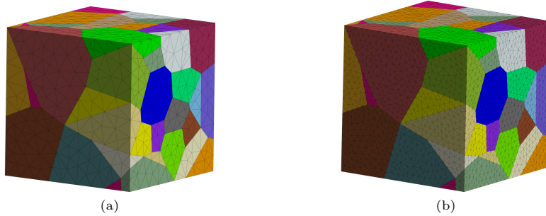
Fig. 10: Computing polycrystals with FE meshes of 64 randomly oriented grains generated by Voronoi tessellation: (a) Coarse (1774 nodes, 8274 elements) and (b) fine (16402 nodes, 85251 elements) meshed. Colors represent the individual grains.
