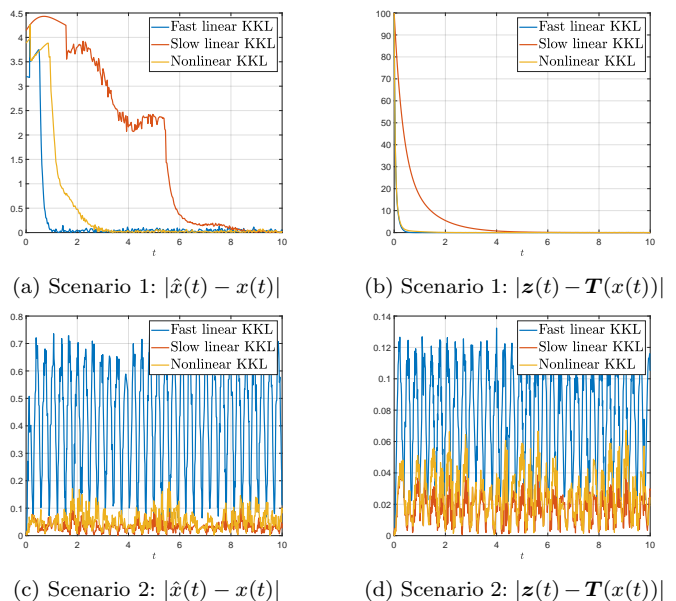
Fig. 1. Estimation error in x and z coordinates from two KKL observers with linear dynamics (2) with slow and fast pairs (A_{\text{slow}}, B_{\text{slow}}) and (A_{\text{fast}}, B_{\text{fast}}) defined from (31), and by a KKL observer with nonlinear dynamics (3) defined from (32). Scenario 1: initial error but no noise; Scenario 2 : no initial error but noise.
