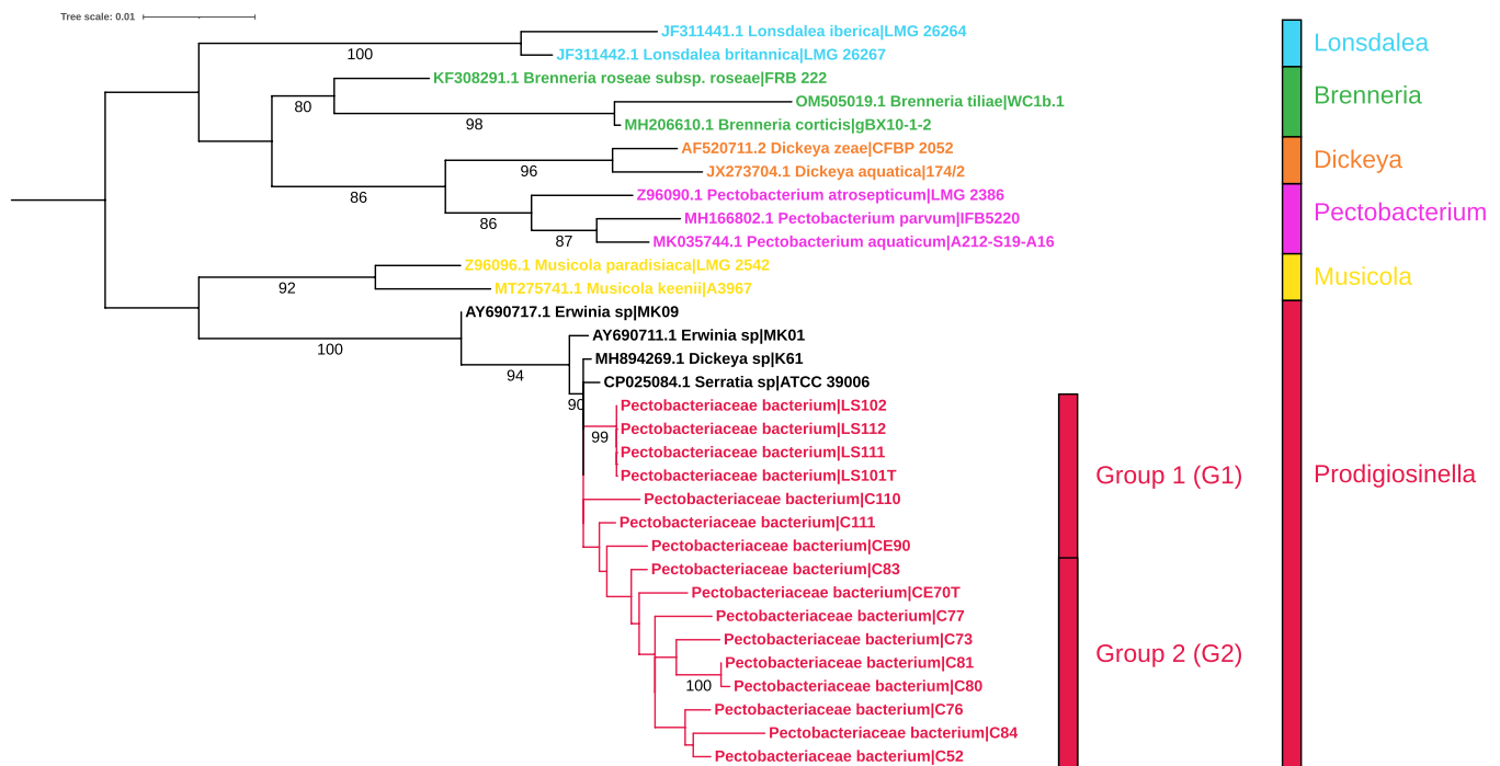
Fig. 3. Maximum likelihood phylogeny of Prodigiosinella strains based on the 16S rRNA gene sequences (32 sequences, 1,468 nucleotide positions). The tree was inferred with IQ-TREE (TN+F+I+G4 model) using sequences of the 16S rRNA PCR products of sixteen strains isolated in Camargue and the available 16S rRNA gene sequences of Serratia sp. ATCC 39006 (CP025084.1), Erwinia sp. MK01 and MK09 (AY690711 and AY690717), Dickeya sp. K61 (MH894269), and a set of Pectobacteriaceae type strains. The scale bar represents the average number of substitutions per site. Numbers at branch represent ultrafast bootstrap values computed with IQ-TREE (1,000 replicates). For clarity values <80 % are not shown.
