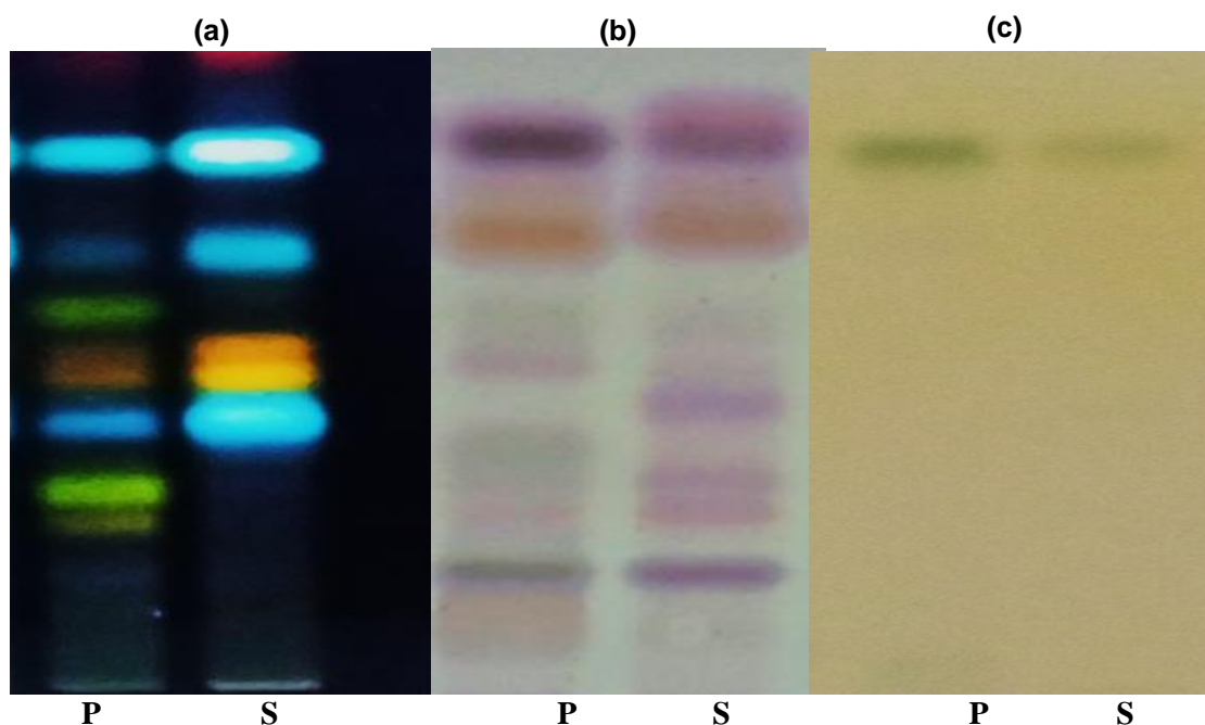
P , pulp; S , seed; (a) , revelation of flavonoids by Neu reagent in the presence of UV light (366 nm); (b) , revelation of sterols and triterpenes in ethanolic (70%) extracts; (c) , revelation of tannins by \text{FeCl}_3 2%.
