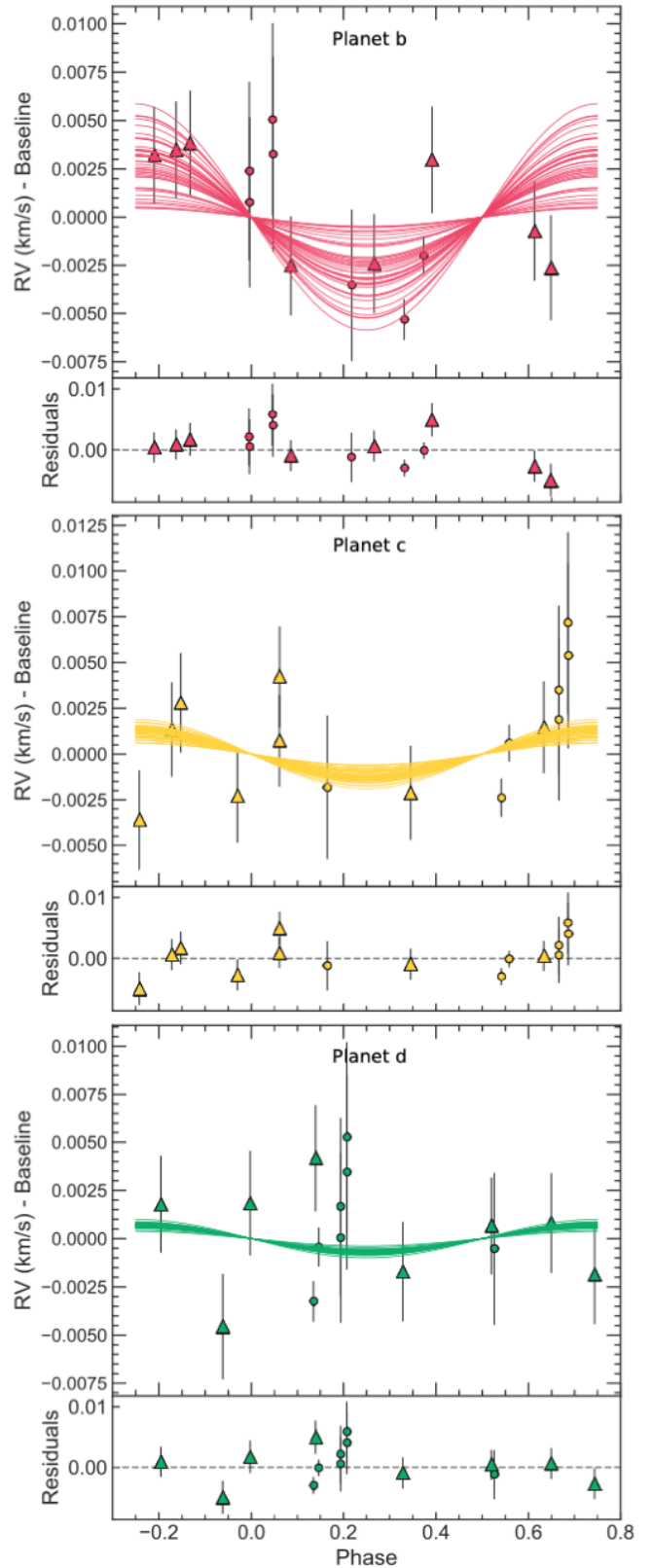
Figure 11. Phased radial velocity measurements for each of the three planets. Triangles are points from ESPRESSO, while circles are points from HARPS; the curves are 20 model samples from the posterior. The data uncertainties include the RV jitter.
