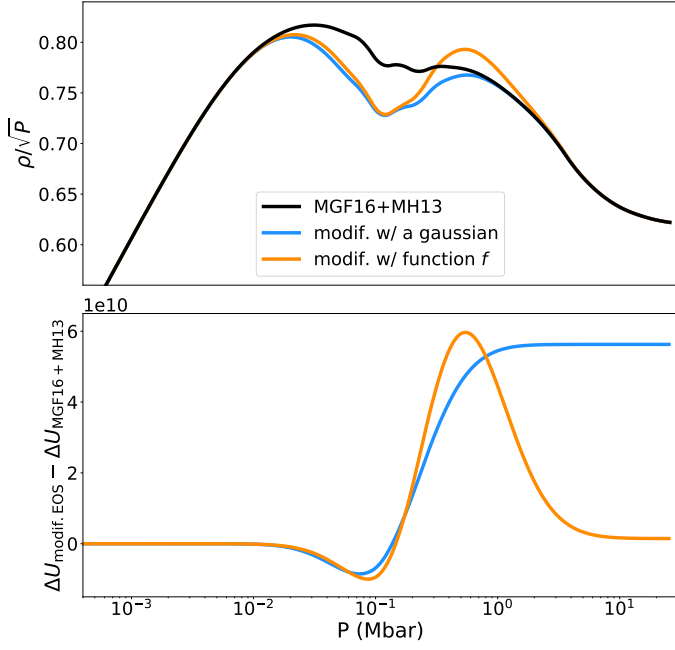
Fig. 5. Comparisons of the \Delta U difference for a model modified with only a Gaussian function (blue) and a model modified with the defined function f (see Eq. (9)) composed of a Gaussian and an error function (orange). Top panel. Comparison of the adiabats ( P_{\text{modif}} = 10^{11} \text{ dyn.cm}^{-2} , \Delta P=0.5 , d\rho=-0.06 for the blue curve & P_{\text{modif}} = 10^{11.5} \text{ dyn.cm}^{-2} , \Delta P=0.6 , d\rho=-0.05 ). Bottom panel. Difference between the \Delta U of the modified models and that of the reference model (MH13).
