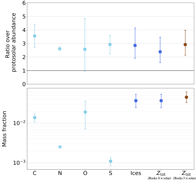
Fig. 1. Abundances of heavy elements in the atmosphere of Jupiter. Here, ‘ices’ refers to the metallicity of the atmosphere considering only ices ( \text{CH}_4 , \text{NH}_3 , \text{H}_2\text{O} and \text{H}_2\text{S} ). Two values of Z_{\text{tot}} are shown, which correspond to the metallicity of the atmosphere considering ices (volatiles) and assuming either no rocks (refractories) or an enrichment of three times the protosolar value for rocks. Abundances of methane and hydrogen sulfide are taken from Wong et al. (2004), and ammonia and water abundances are taken from Li et al. (2020). Protosolar abundances are taken from Asplund et al. (2021). The protosolar mass fraction of heavy elements is 0.0154. For ices, we calculated the protosolar value considering C, N, O, S, and Ne and included additional elements with the value from Lodders et al. (2009). Concerning rocks, we only considered Mg, Si, and Fe.
