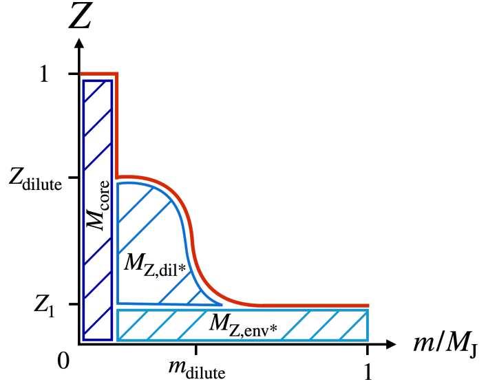
Fig. 2. Distribution of heavy elements for a model with a dilute core. The three hashed areas correspond to the mass of the compact core (only made of heavy elements), the mass of heavy elements in the dilute core region excluding the area where Z < Z_1 , and the mass of heavy elements in the rest of the envelope (where Z < Z_1 ). Z_1 is the mass fraction of heavy elements in the outer envelope. Z_{\text{dilute}} is the maximum mass fraction in the dilute core. m_{\text{dilute}} monitors the extent of the dilute core in terms of mass.
