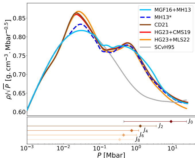
Fig. 3. Adiabats obtained from different EOSs and corresponding to a homogeneous model, with no compact core, with Y = 0.245 . Table 1 lists the details of the EOSs. Below are shown the contribution functions of the gravitational moments of order 0 to 8 centred at their peak. Their extent corresponds to their full width at half maximum (see Guillot (2005) for more details).
