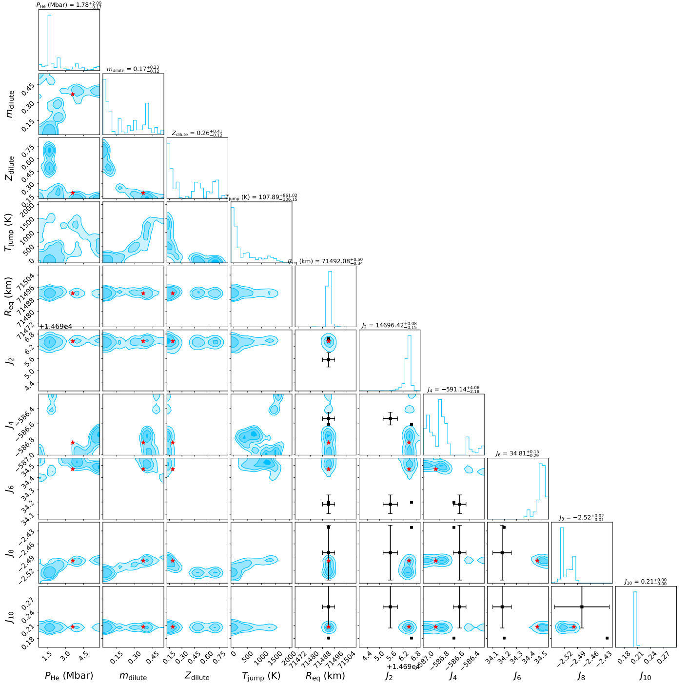
Fig. D.1. Posterior distributions obtained with MH13*. The red star shows the Miltzer et al. (2022) preferred (static) model. M_{\text{core}} = 0 , T_{1\text{bar}} is fixed at 166.1 K and Z_1 = 0.0153 . The black error bars correspond to Juno's measurements accounting for differential rotation for the J_{2n} .
