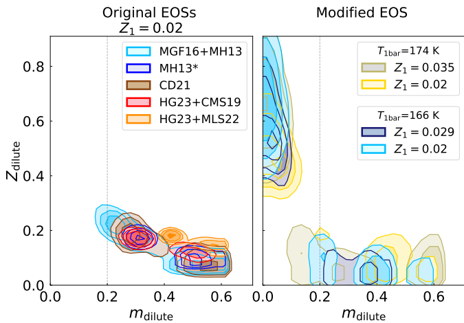
Fig. 13. Z_{\text{dilute}} vs. m_{\text{dilute}} for two types of models. Z_{\text{dilute}} is the maximum mass fraction of heavy elements in the dilute core region while m_{\text{dilute}} controls the extent of the dilute core in terms of mass (see Section 2.2). Left panel. Models using original EOSs. Z_1 = 0.02 . Right panel. Models with a modification of the EOS. The initial EOS that has been modified is MH13. We present two subsets of models: with T_{1\text{bar}} = 166.1 K and T_{1\text{bar}} = 174.1 K. The thin gray dotted line corresponds to m_{\text{dilute}} = 0.2 , which corresponds approximately to the extent of the dilute core of 20% of Jupiter’s mass predicted by formation models from Müller et al. (2020).
