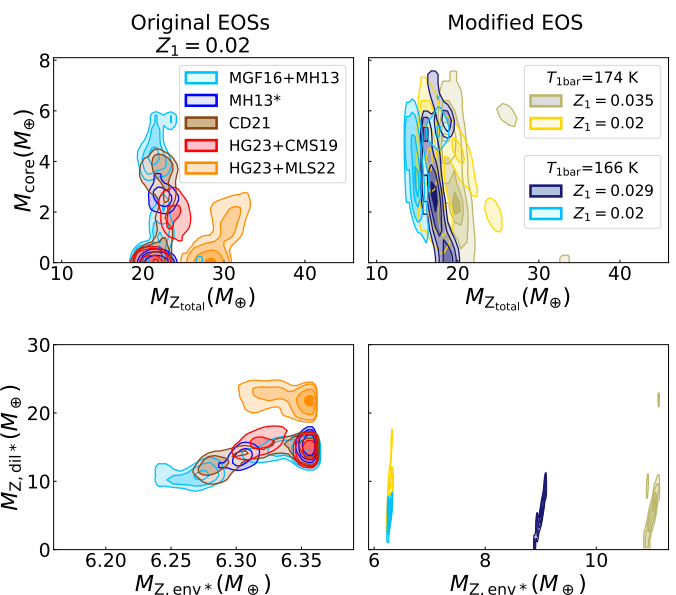
Fig. 12. Masses of heavy elements in our interior models. Top panels. Mass of the compact core vs. total mass of heavy elements in Jupiter. Bottom panels. M_{Z,\text{dil}*} vs. M_{Z,\text{env}*} (see Section 2.2).
