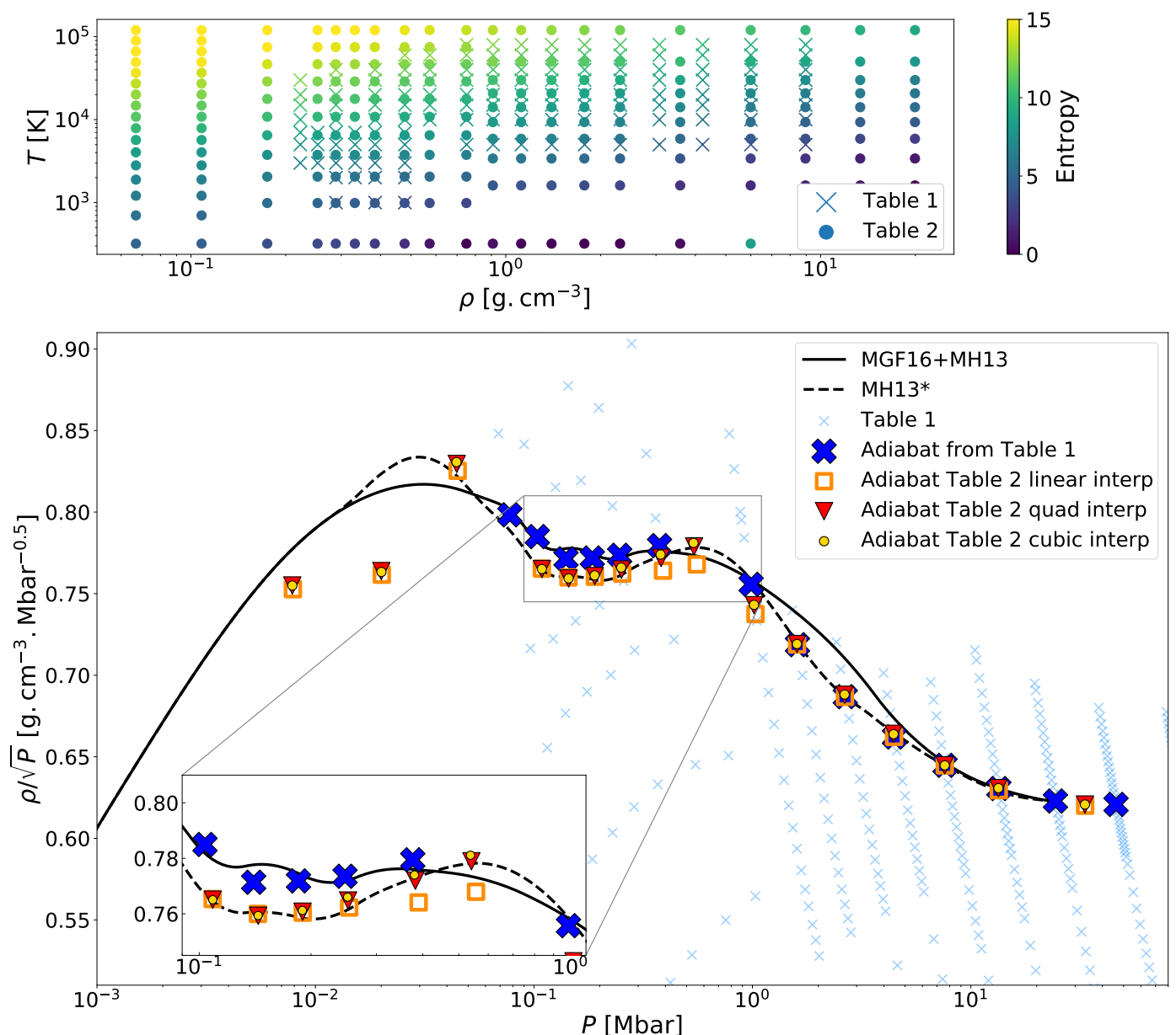
Fig. 4. Comparison between the MH13* and MGF16+MH13 EOSs. Top panel. Comparison of Table 1 and Table 2 from Militzer & Hubbard (2013). Bottom panel. Comparison of adiabats obtained with the MH13* and MGF16+MH13 EOSs and of points obtained by direct interpolation of the above tables. The (P, \rho/\sqrt{P}) points of Table 1 from Militzer & Hubbard (2013) are shown as blue crosses. The locations at which the entropy is equal to 7.078061 k_{\text{B}} \text{el.}^{-1} (a typical value of entropy for Jupiter) according to the interpolations in the two tables are shown with different symbols, as labelled.
