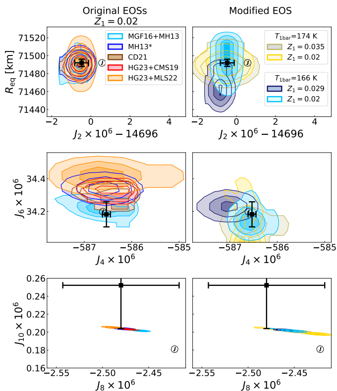
Fig. 11. Equatorial radius and gravitational moments for two types of models. Left panels. Models using original EOSs. Z_1 = 0.02 . Right panels. Models with a modification of the EOS. The initial EOS that has been modified is MH13. We present two subsets of models: with T_{\text{1bar}} = 166.1 K and T_{\text{1bar}} = 174.1 K. The circles with a J correspond to the measurements of the gravitational moments by Juno (Durante et al. 2020). The black error bars correspond to the gravitational moments corrected by differential rotation (see 2.1).
