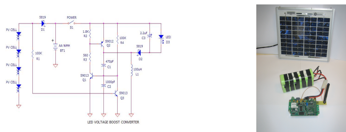
Figure 7: A boost circuit added to the PEGASE concept for an optimal solar cells source
