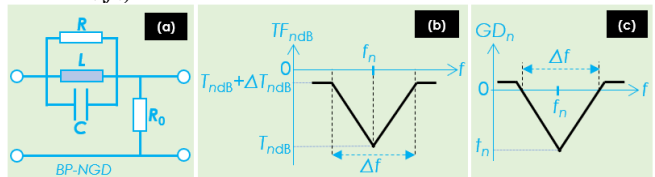
Fig. 3. BP-NGD (a) equivalent circuit, (b) TF_n and (c) GD_n specifications.
