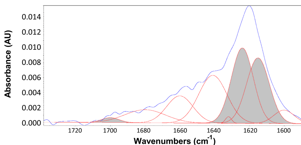
Assignment of the protein structure contributions to amide I band (1580–1720 \text{cm}^{-1} )
