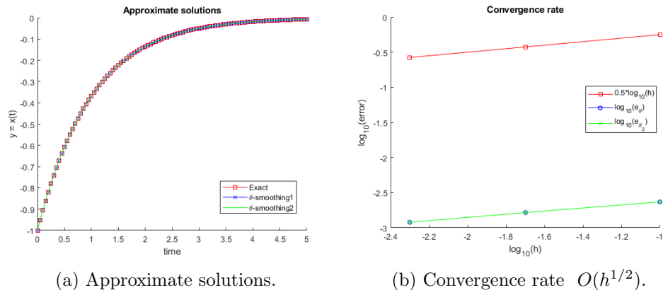
Figure 2: Solving equation 3.5
