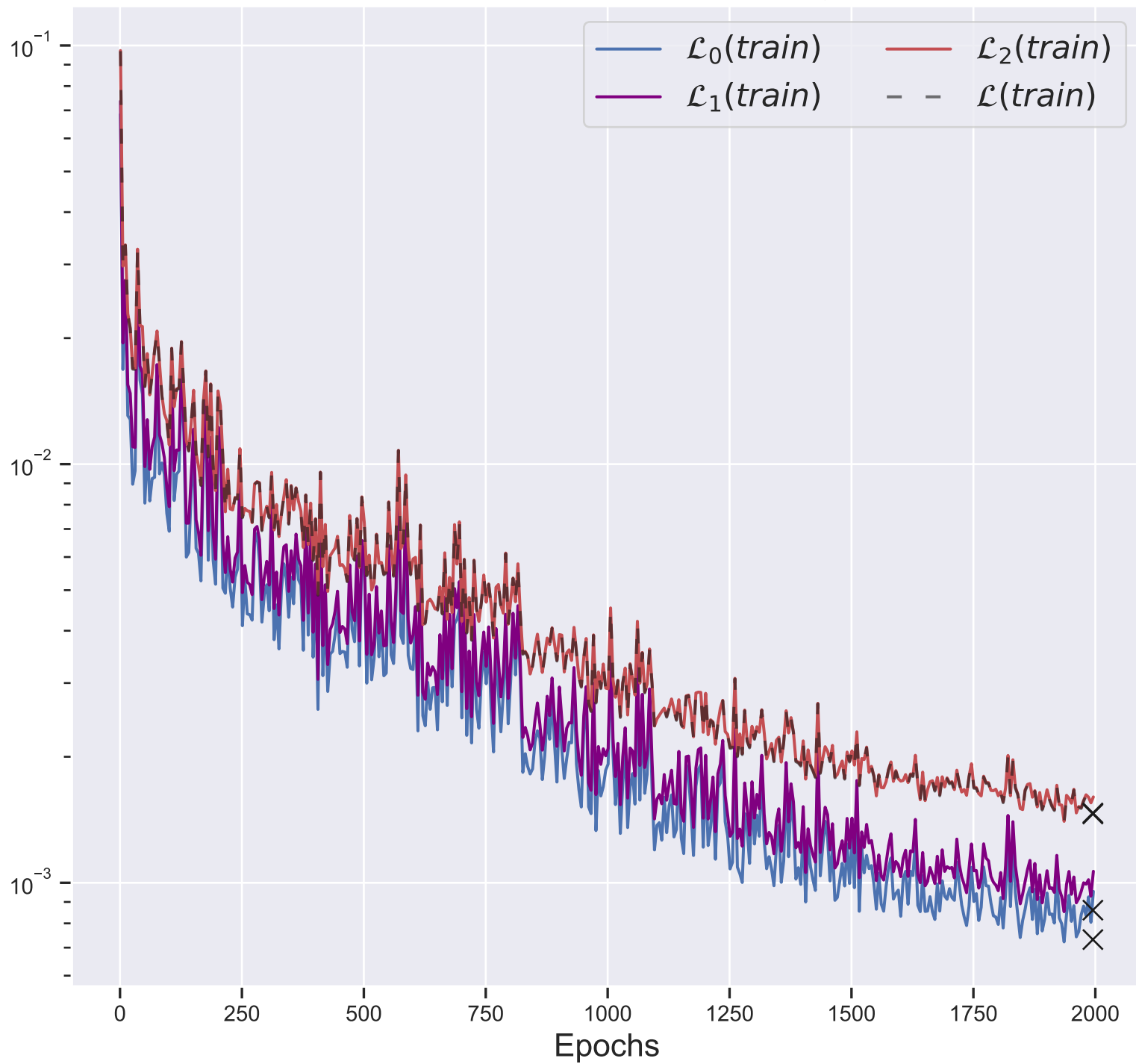
Evolution of \mathcal{L} and \mathcal{L}_i on the training set
