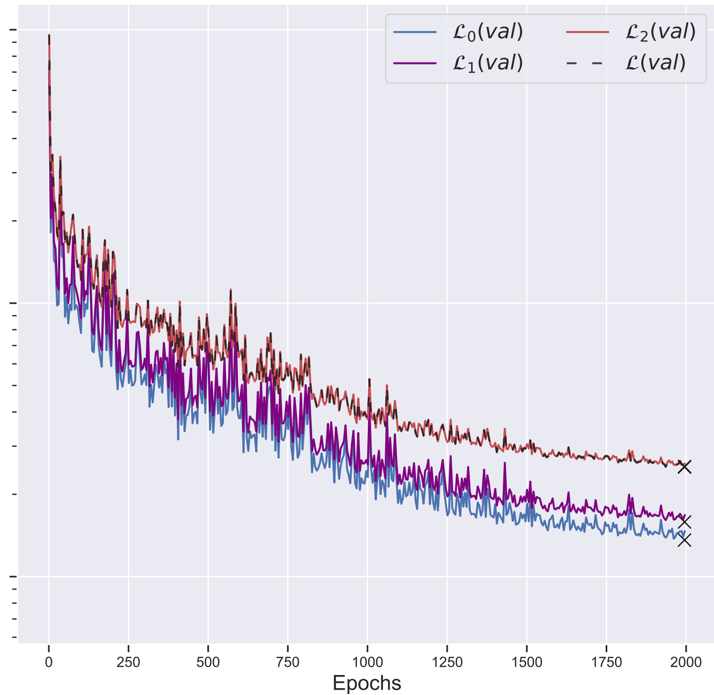
Evolution of \mathcal{L} and \mathcal{L}_i on the validation set
