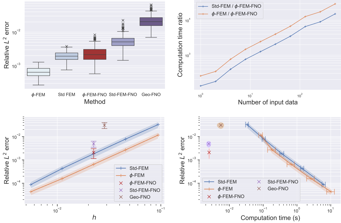
Figure 11: Test case 1. Top left: Relative L^2 errors of the methods (from left to right: \phi -FEM, standard method, \phi -FEM-FNO, Standard-FEM-FNO, Geo-FNO). Top right: computation times of the methods. Bottom left: Relative L^2 errors, with respect to h . Bottom right: Relative L^2 errors, with respect to the computation times.
