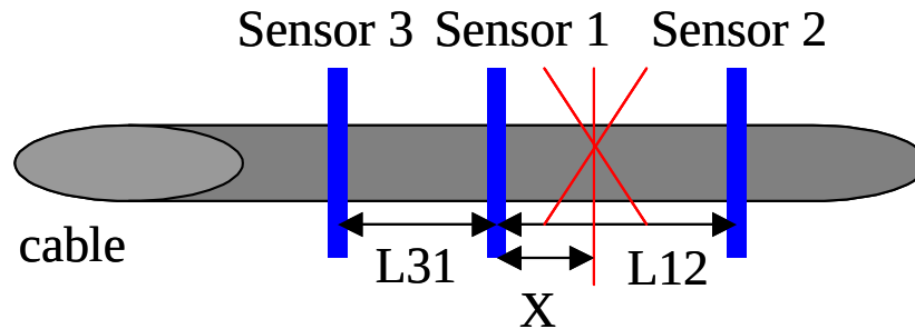
Figure 2. Rupture localization by acoustic sensors
