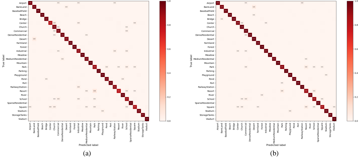
Fig. 8. Confusion matrix (CM) on AID dataset. (a) 20% of the dataset for training and the rest for testing. (b) 50% of the dataset for training and the rest for testing.
