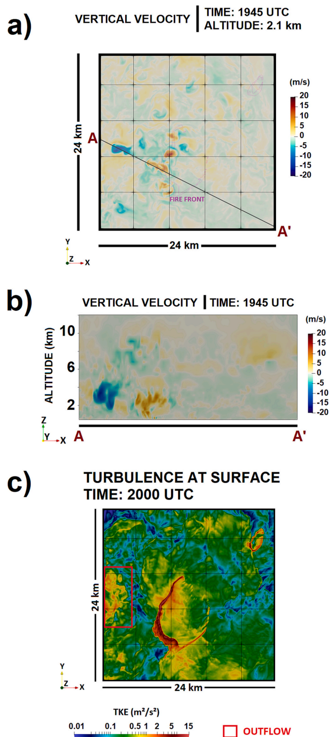
Fig. 10. a) Vertical velocity at 2.1 km altitude at 1945 UTC, b) A-A' vertical cross-section indicated in Fig. 10a with vertical velocity (m/s) at 1945 UTC, and c) turbulent kinetic energy ( \text{m}^2/\text{s}^2 ) at surface at 2000 UTC. The purple contour in Fig. 10a represents the fire front. (For interpretation of the references to colour in this figure legend, the reader is referred to the web version of this article.)
