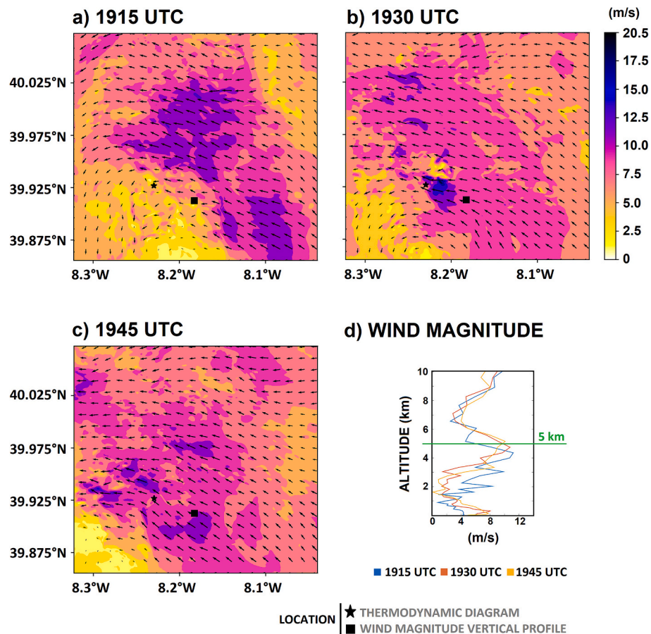
Fig. 12. Wind magnitude (coloured areas; m/s) and direction (arrows) at 5 km altitude a) at 1915 UTC, b) at 1930 UTC, and c) at 1945 UTC; d) Vertical profile of horizontal wind magnitude (m/s). The symbols in Fig. 12a – c indicate the location used to plot the thermodynamic diagram and the vertical profile of wind magnitude.
