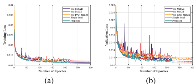
Fig. 11. Convergence curves for different network structures. (a) Training loss curves. (b) Validation loss curves. Please note that the single-level loss is calculated by (8), while the loss of the other structures is calculated by (6) (with \gamma = 0.4 ). Please note that the learning rate for 0-220 epochs is 0.001, and for 220-300 epochs is adjusted to 0.0001.
