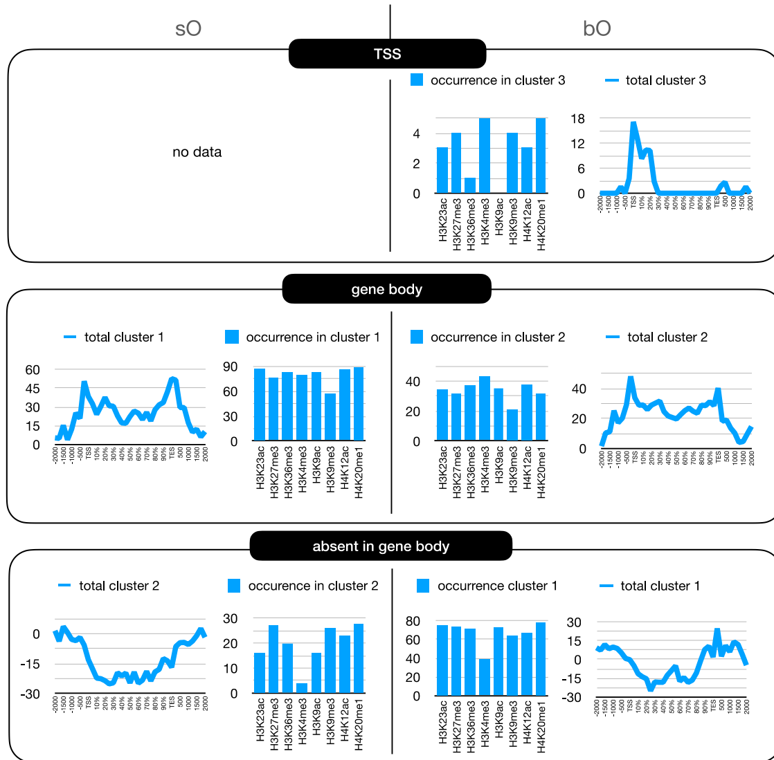
Fig. 1b. Metagene profiles of ovaries of single sex, pairing-unexperienced females (sO), and bisex, pairing-experienced females (bO). Axis as for figure 1a.
