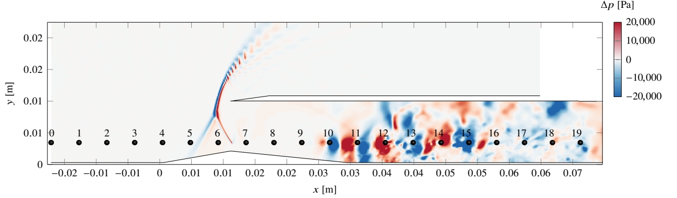
Figure 10 Instantaneous field of the fluctuating pressure \Delta p = p - \bar{p} in the z = 0.005 plane. (Black spheres) Probe number and location along the air inlet.
