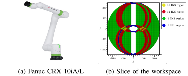
Fig. 5: Fanuc CRX 10iA/L and a slice of its workspace for y = 0.05 m and orientation represented as Tait-Bryan angles \alpha_o = 0.153^\circ , \beta_o = 0.639^\circ , \gamma_o = 0^\circ .
