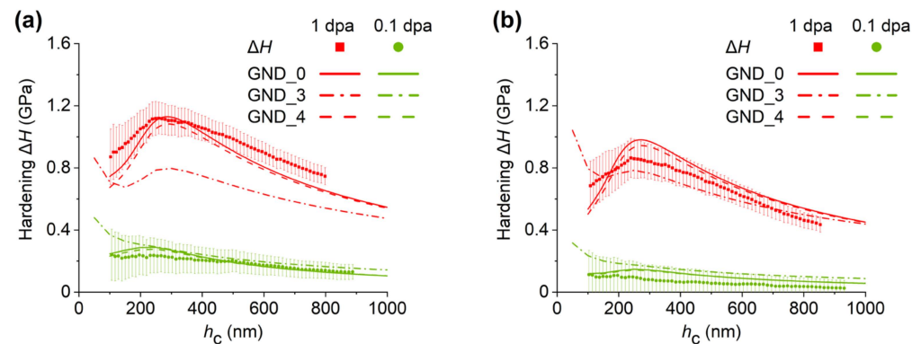
Figure 12. Case 4 model predictions with experiments for (a) ANP-6 and (b) ANP-10.
