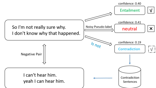
Figure 1: A conceptual illustration of contrastive negative learning. For a low-confidence target sample (top left), the model is uncertain between the wrong label (marked in red) and the ground truth label (marked in green), and produce a noisy pseudo-label. In contrast, the complementary label (marked in blue) is often correct about “the sample does not belong to the class” and thus provides class-wise contrastive information (bottom left).
