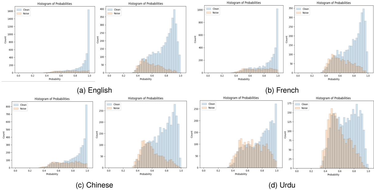
Figure 3: Noise rate change before and after the contrastive negative learning stage of four languages. Bins in blue indicate clean samples while bins in orange indicate noisy samples. The horizontal axis indicates the confidence score of the samples calculated using the model’s predicted class distribution; the vertical axis indicates the number of samples falling in the area of confidence.
