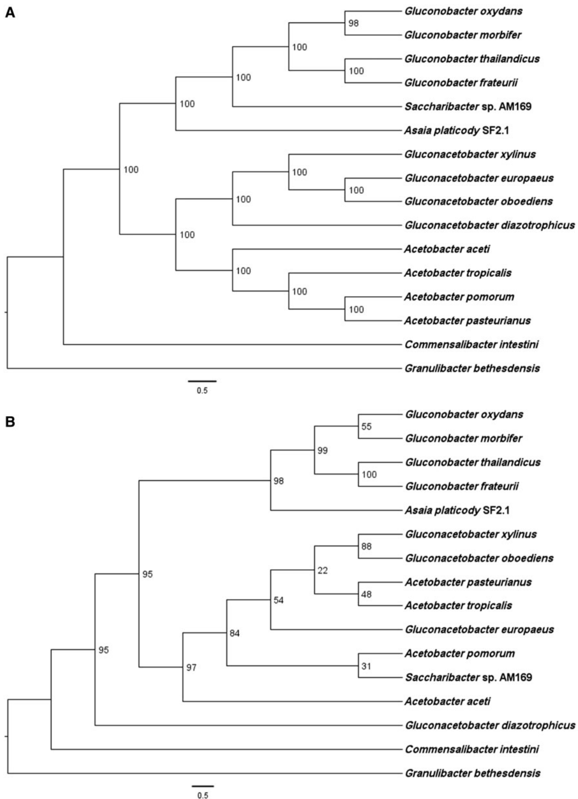
Fig. 2. —Comparison of species (AAB) (A) and operon (cytochrome oxidase bc ) (B) in phylogenetic trees. The scientific names at the terminal nodes are those of the bacteria species. The tree of AAB (top) is based on the results of 70 concatenated protein (supplementary table S1, Supplementary Material online) phylogenetic analyses. Operon tree (bottom) was derived from the phylogeny inferred from the bc operon. The tree topology and other details were as given in figure 1.
