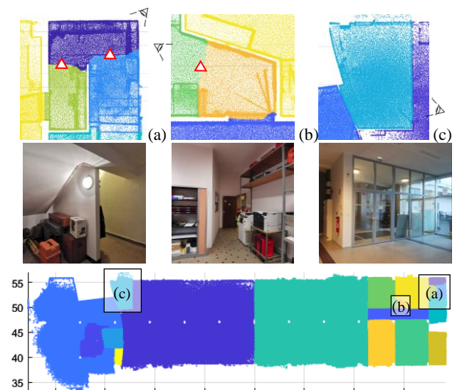
Figure 10. INSA-0 point cloud segmented into rooms. Red triangles localise over-segmentations. (a) and (b) focus on over-segmentation locus, and (c) on glazed walls.
