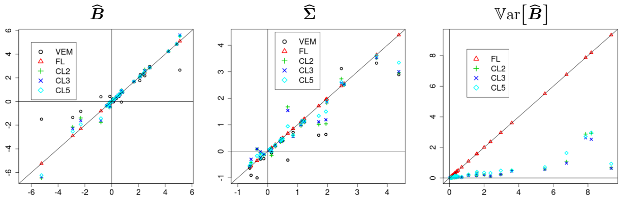
Figure 6: Comparison of the estimates with the different algorithms. Left: regression coefficients \widehat{\beta}_{hj} , center: covariance parameters \widehat{\Sigma}_{jk} , right: estimated variances of the regression coefficients \widehat{\beta}_{hj} . x -axis = full likelihood inference (FL), y -axis: likelihood inference (FL = red triangle \triangle = reference), composite likelihood inference (CL2 = green plus + , CL3 = blue times symbol \times , CL5 = cyan diamond \diamond ) and variational EM (VEM = black circles 'o').
