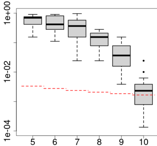
Figure 9: Distribution of the p -values of the Kolmogorov-Smirnov test for the distribution of the standardized estimates \tilde{\beta}_{\ell j} (over the M = 100 simulations) as a function of the number of species ( p = 5, \dots, 10 ) for full-likelihood inference (FL). Dotted red lines: \alpha = 5\% significance threshold after Bonferroni correction ( i.e. , \alpha/(dp) ).
