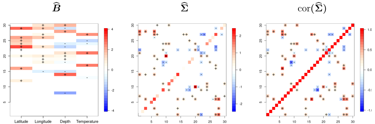
Figure 8: Colormap of the parameter estimates. Left: regression coefficients \widehat{\beta}_{\ell j} , center: covariance parameters \widehat{\sigma}_{jk} , right: corresponding correlations \widehat{\rho}_{jk} = \widehat{\sigma}_{jk} / \sqrt{\widehat{\sigma}_{jj} \widehat{\sigma}_{kk}} . Blank cells correspond to non-significant estimates, red cells (marked with '+') to positive estimates and blue cells (marked with '-') to negative estimates.
