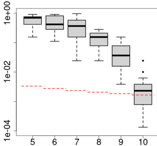
Figure 9: Distribution of the p -values of the Kolmogorov-Smirnov test for the distribution of the standardized estimates \tilde{\beta}_{lj} (over the M = 100 simulations) as a function of the number of species ( p = 5, \dots, 10 ) for full-likelihood inference (FL). Dotted red lines: \alpha = 5\% significance threshold after Bonferroni correction ( i.e. , \alpha/(dp) ).
